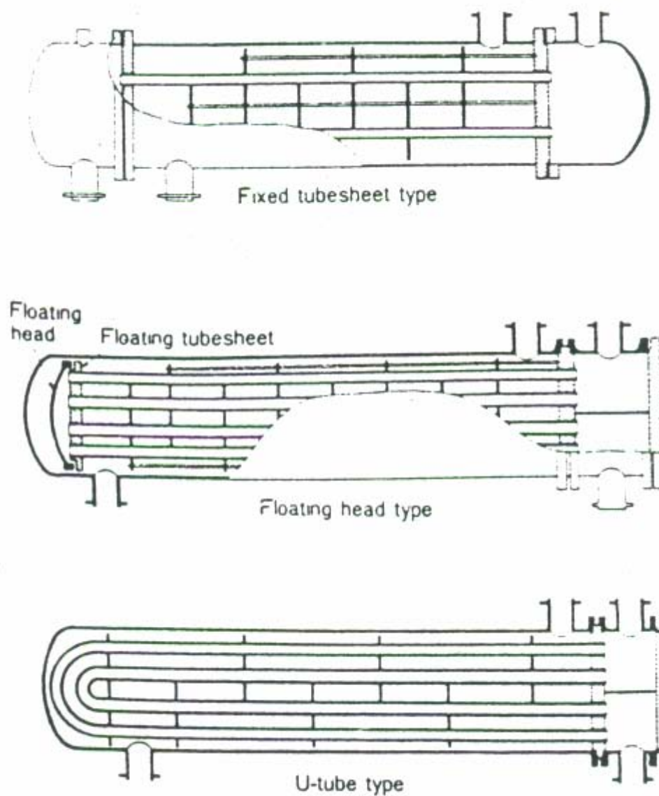
Fig.9 Typical structure of tubular heat exchangers
