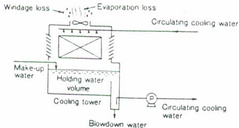
Fig.-10 Water balance in an open recirculating cooling water system
